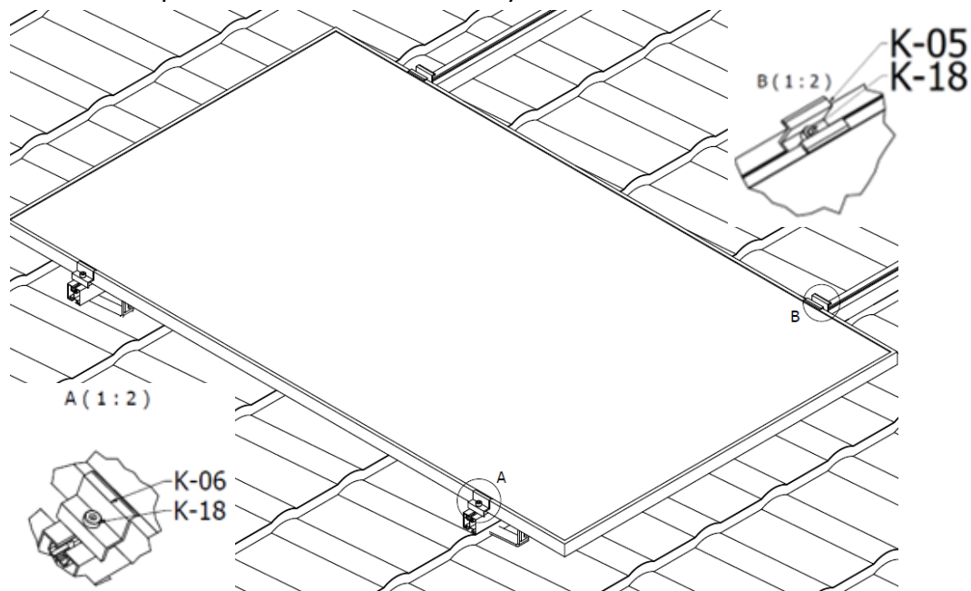
FIGURE. 15 Mounting of the modules and mounting the K-05 and K-06 clamps
