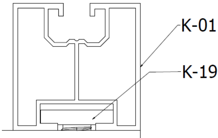
FIGURE. 10 Mounting of profile K-01
