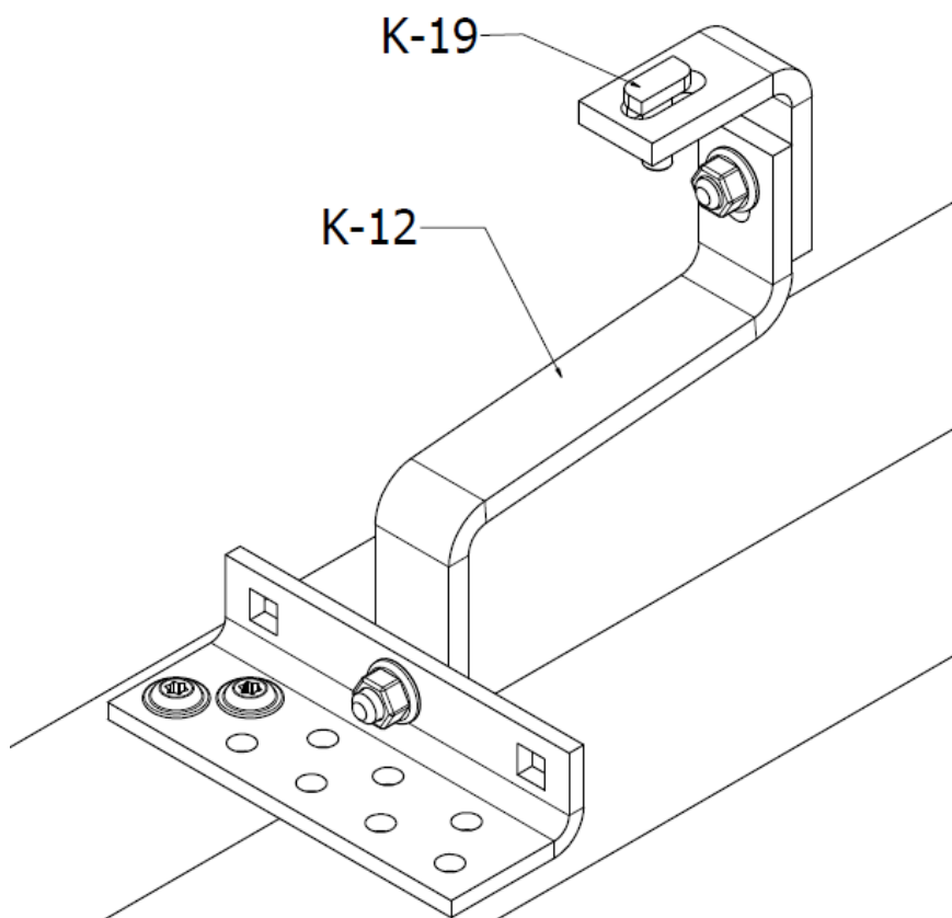
FIGURE. 9 Mounting of "T" bolts
