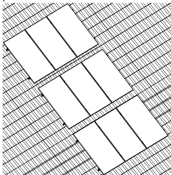
FIGURE. 16 View of assembled structure with modules
