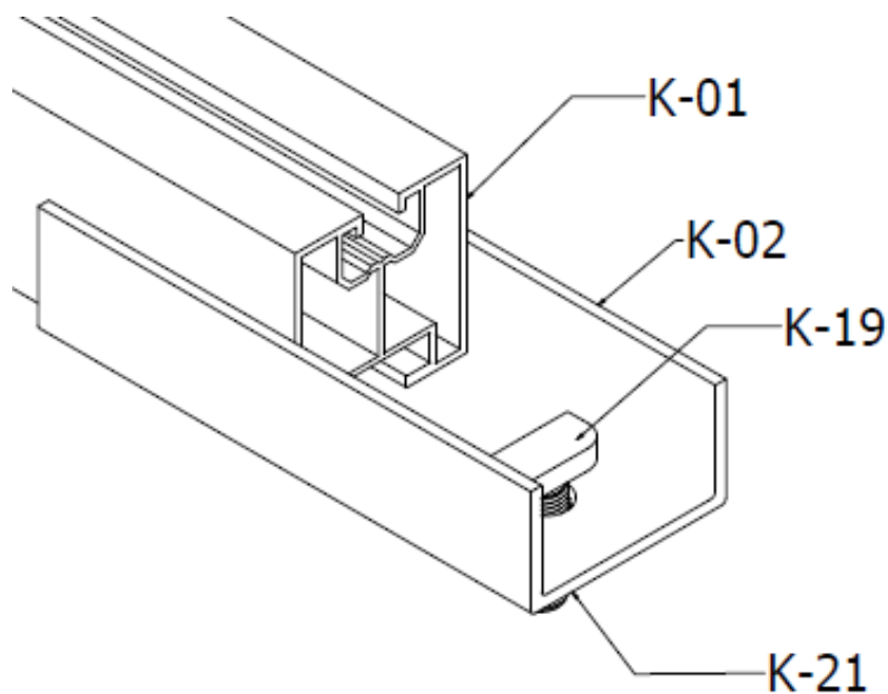
FIGURE. 7 Mounting of the K-02 connector with the K-01 profile
