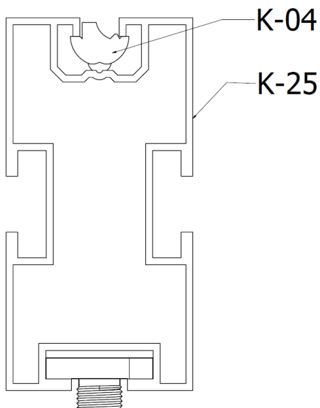
FIGURE. 14 Mounting of the K-04 nut to K-01 profiles
