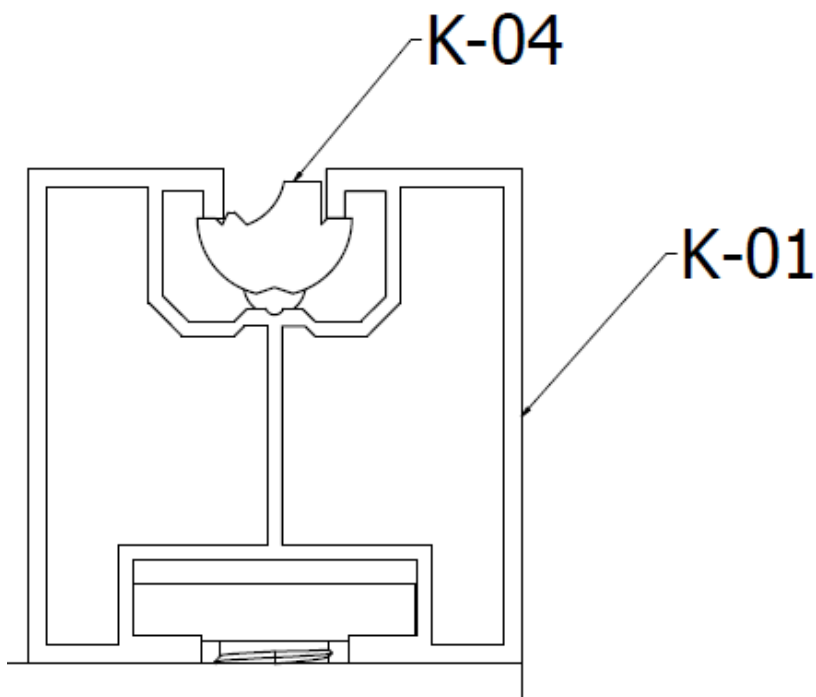
FIGURE. 13 Mounting of the K-04 nut to K-01 profiles
