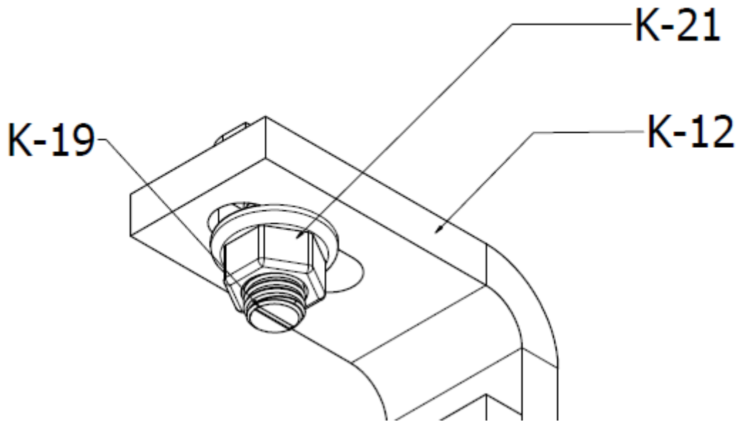
FIGURE. 12 Mounting of "T" bolts
