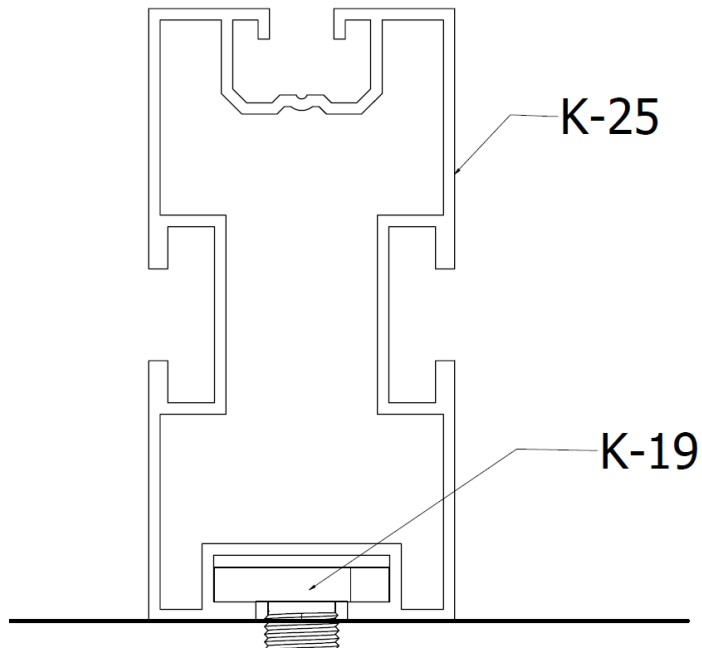
FIGURE. 11 Mounting of profile K-25
