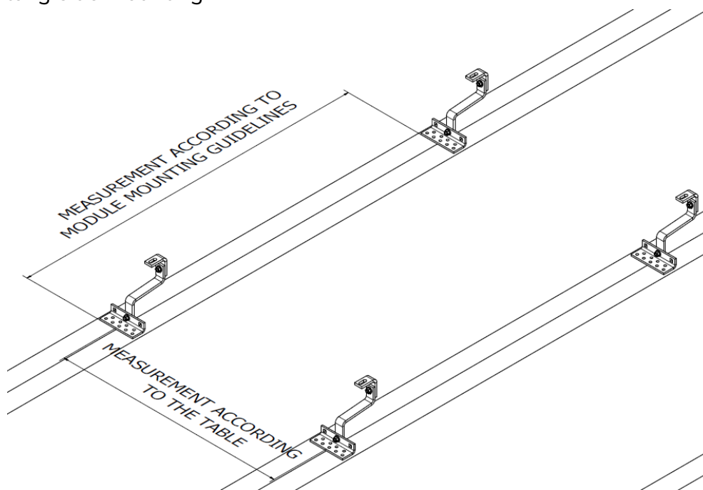
FIGURE. 4 Bracket spacing
