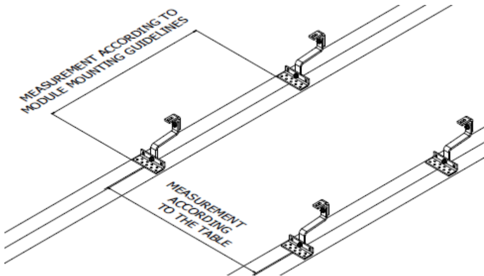
FIGURE. 5 Bracket spacing
